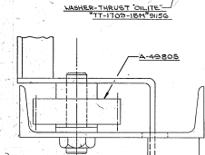
LIMIT SWITCH ASSY.
