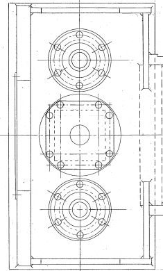
SECTION 13-13
