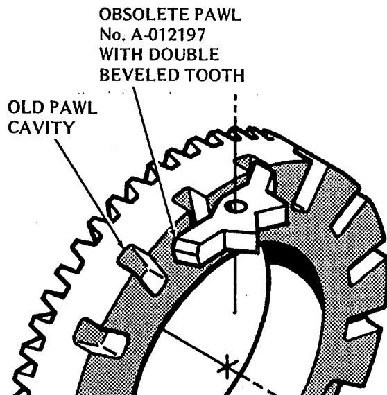
OBSOLETE PAWL & BEVEL GEAR
