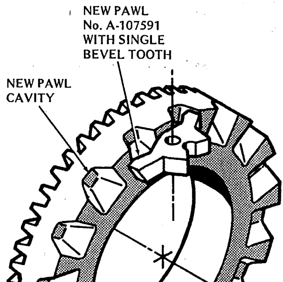
NEW PAWL & BEVEL GEAR
