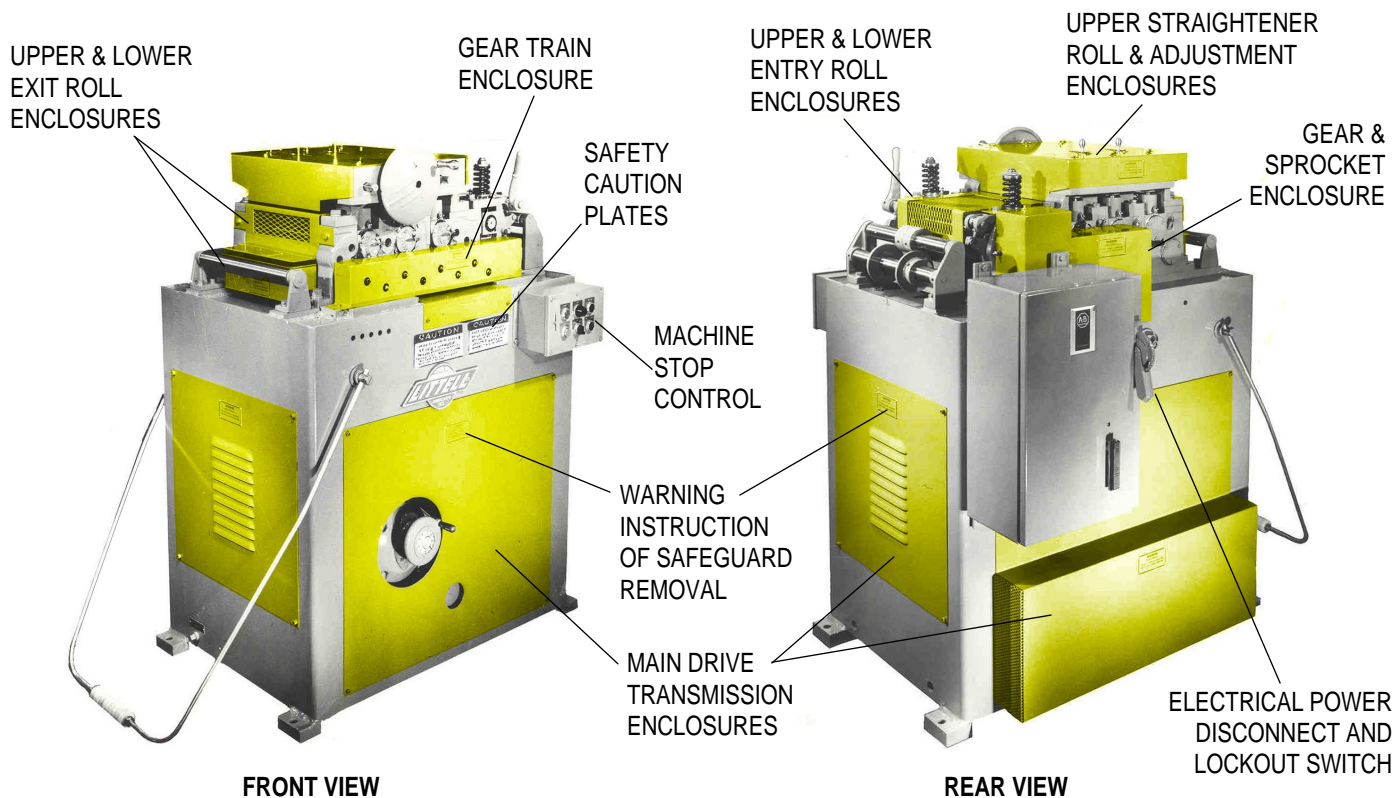
No. 4 STRAIGHTENER
